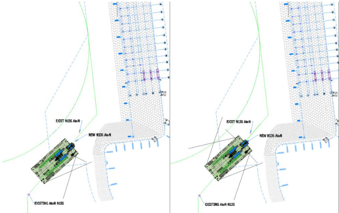
Figure 1 General Barge Position & Anchor Layout During AtoN Installation
