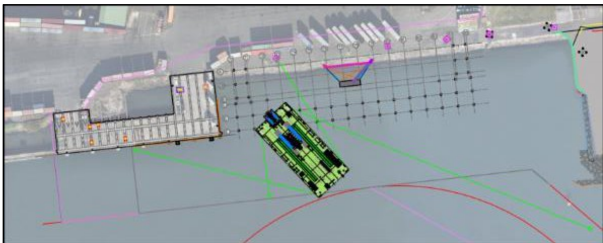
Typical mooring and vessel location 1
